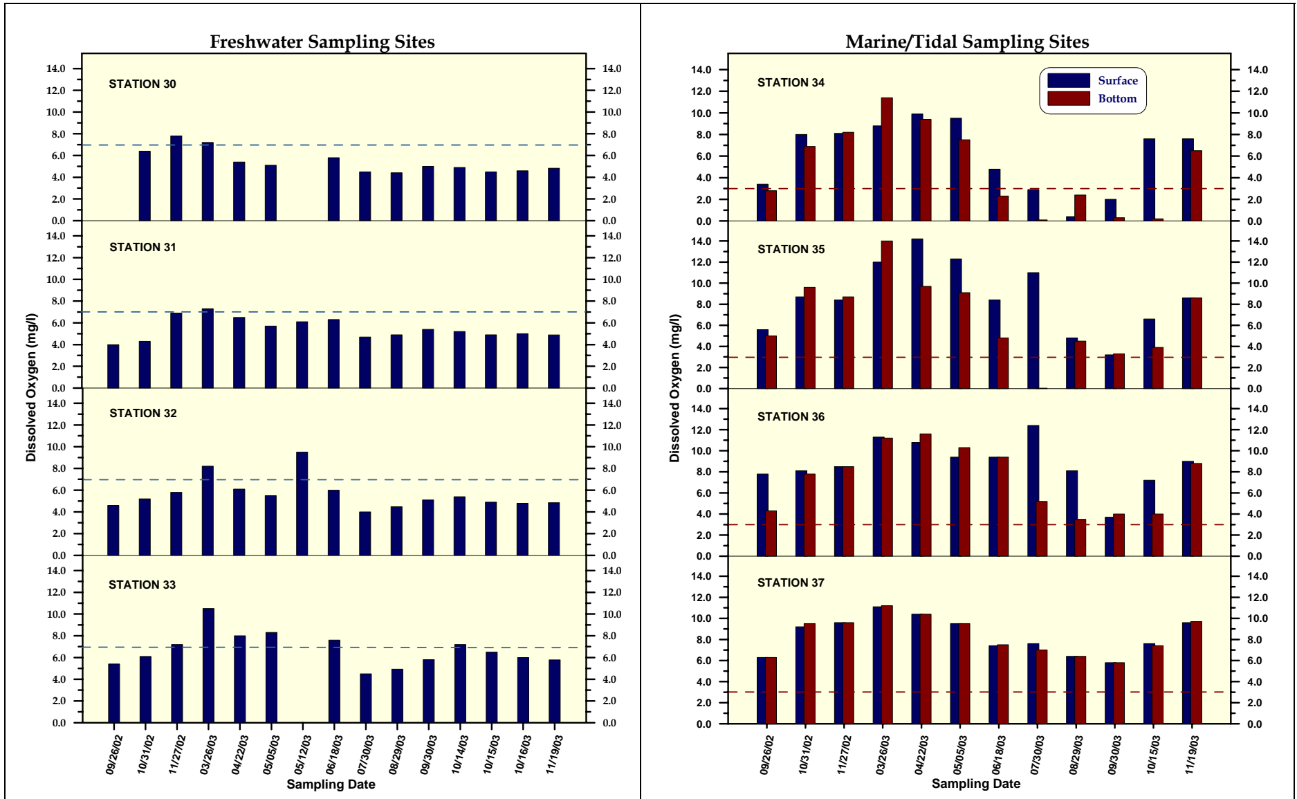
Figure 6. Temporal Variations in Dissolved Oxygen Concentrations, 9/02 – 11/03 (light blue dashed-line is 7.0 mg/l NYS standard for C(TS) waters; red dashed-line is 3.0 mg/l acute standard for SC waters)
