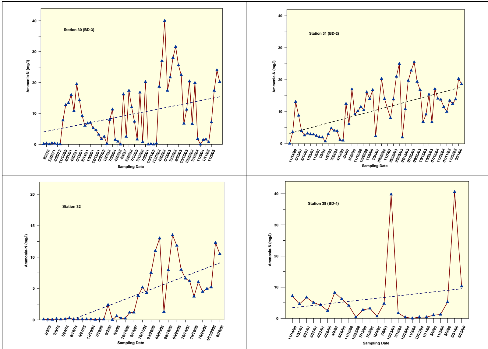
Figure 12. Plots of Historic Ammonia Concentrations at Beaver Dam Creek Stations 30, 31, 32 & 38 Data from SCDHS Office of Ecology and Office of Water Resources, 1970-2006; USGS, 1982; Cashin Associates and Dvirka & Bartilucci, 1989-2005 (Dashed lines are linear trends; note that x-axis dates are not proportionately spaced)
