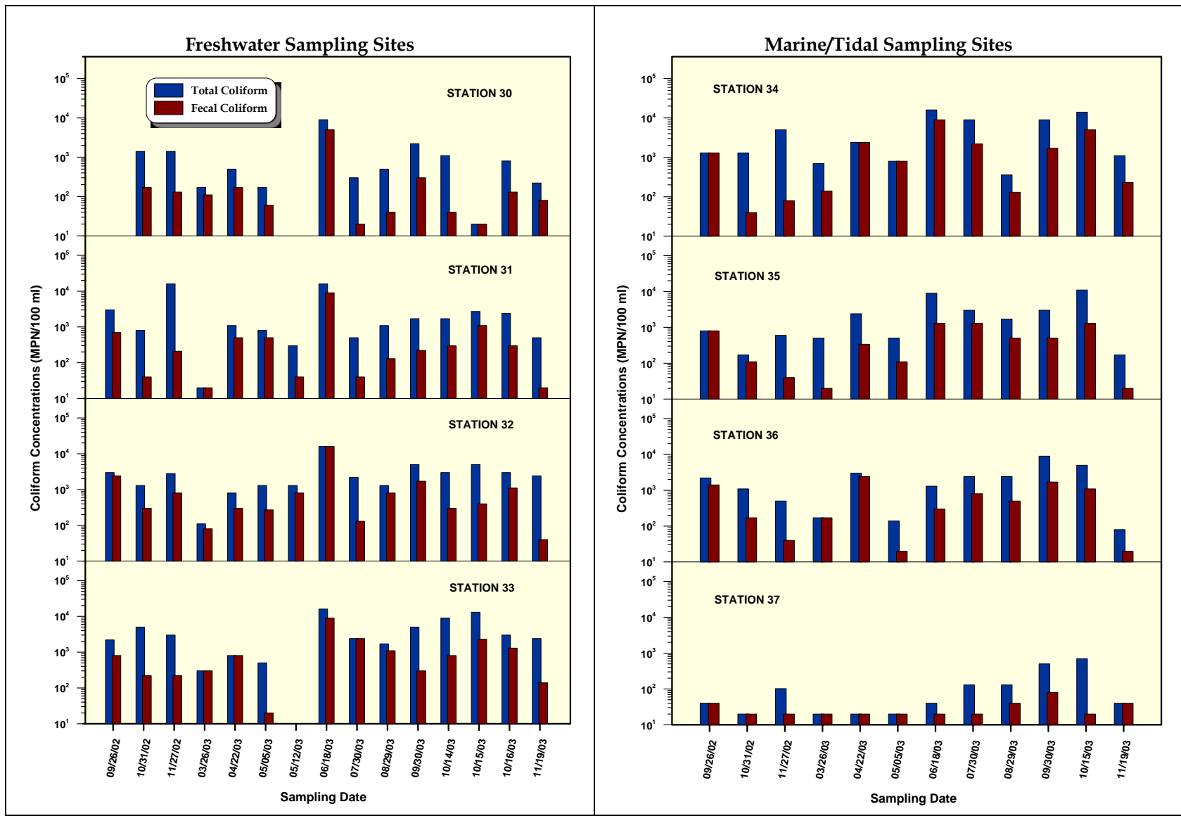
Figure 8. Temporal Variations in Total & Fecal Coliform Concentrations (9/02 – 11/03)
