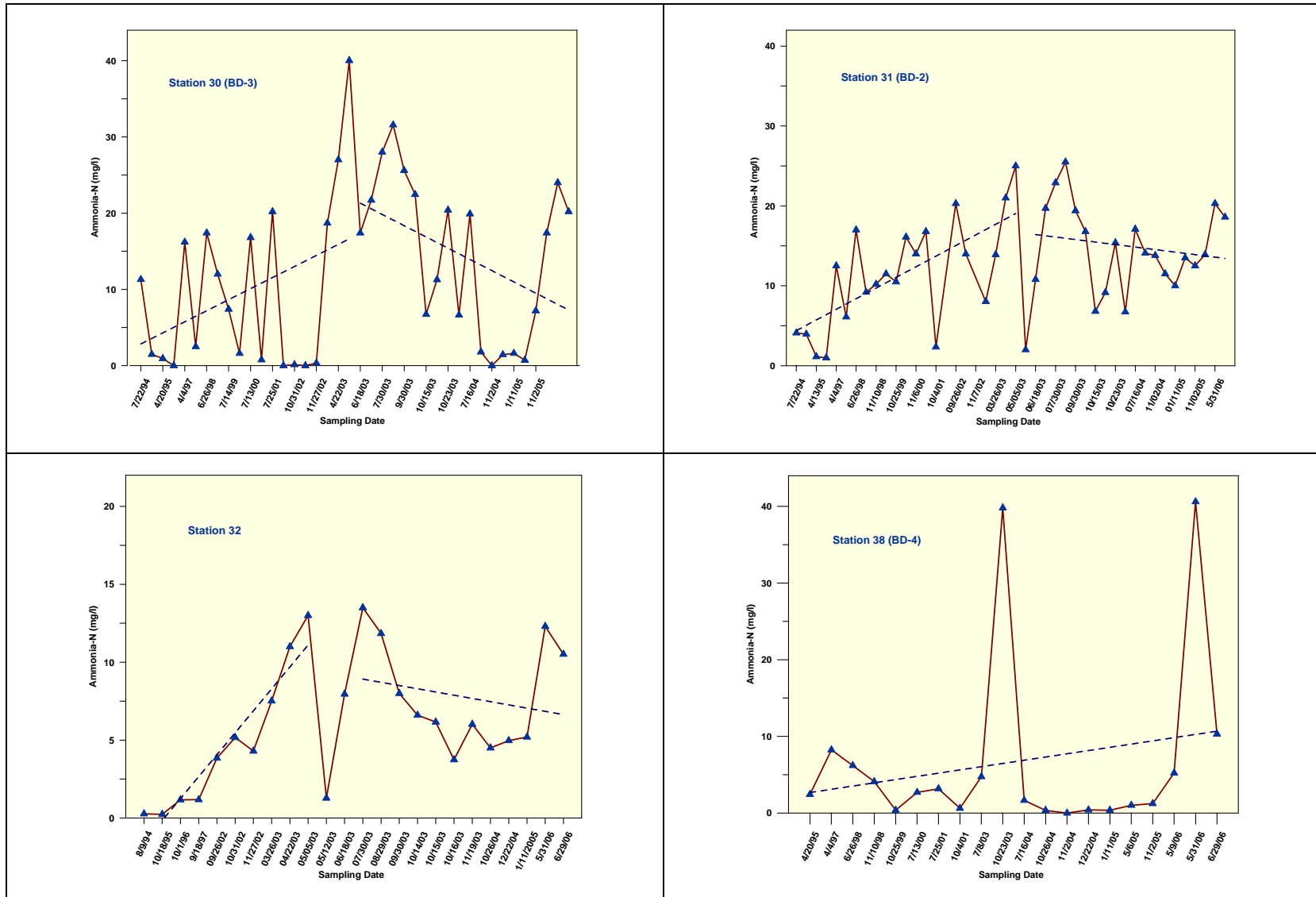
Figure 16. Plots of Post-Closure (1994-2006) Ammonia Concentrations at Beaver Dam Creek Stations 30, 31, 32 & 38 (Dashed lines are linear trends; note date intervals are not uniform)
