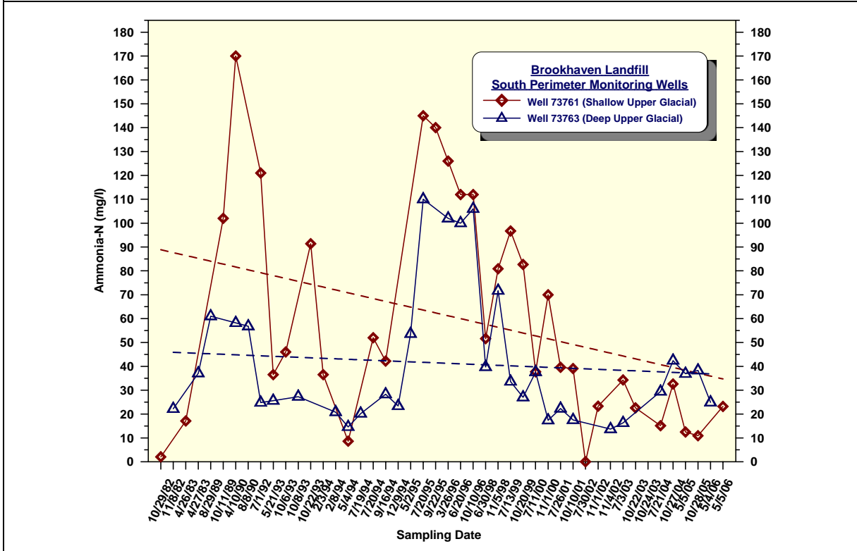
Figure 15. Historical Ammonia Levels in Perimeter Monitoring Wells South of the Brookhaven Town Landfill
