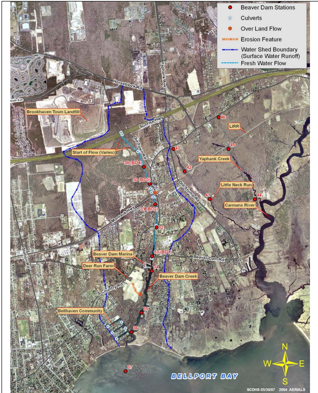
Figure 2. Beaver Dam Creek Stormwater Discharge Locations and Watershed Boundary (from Suffolk County Soil and Water Conservation District GIS Coverages, 2002)
